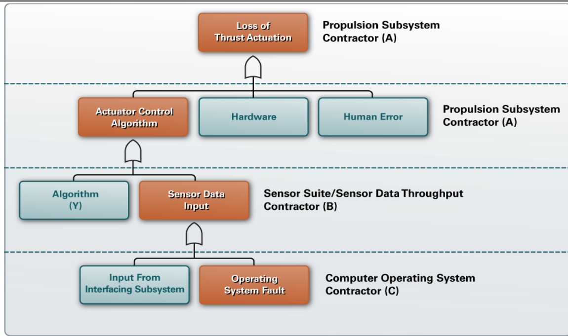
Figure 4-41: Example of a SHA Interface Analysis
